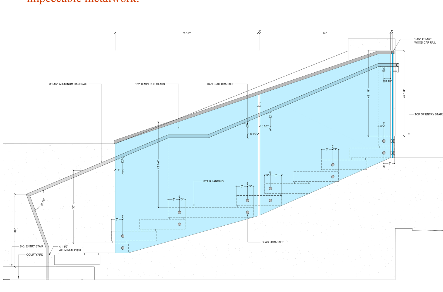
2 ELEVATION 3/4" = 1'-0"
