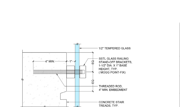
4 DETAIL 3" = 1'-0"
