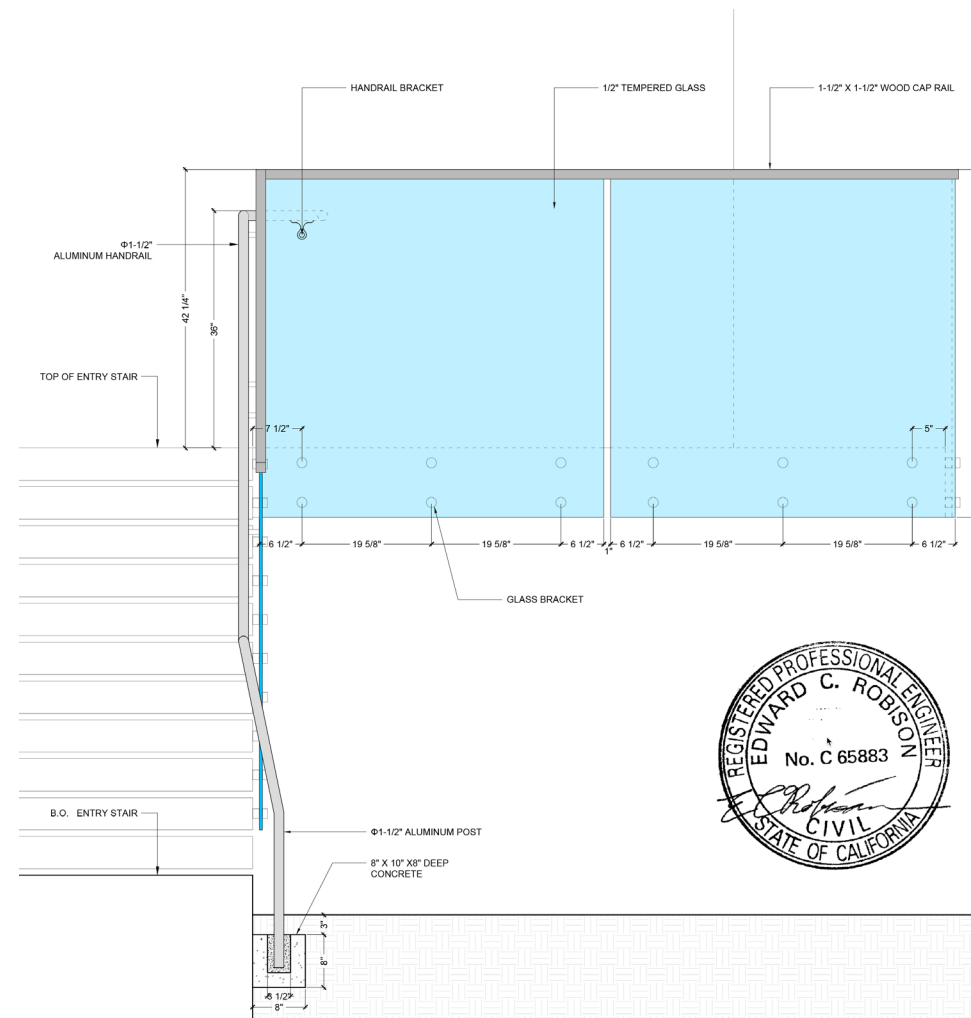
3 ELEVATION 3/4" = 1'-0"
