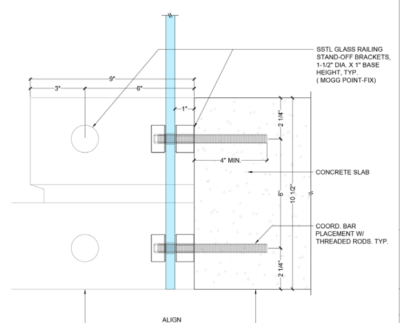
5 DETAIL 3" = 1'-0"
