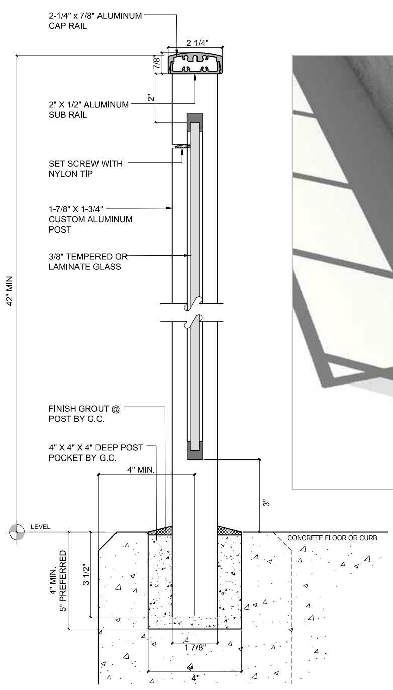
3 SECTION DETAIL - POURED IN PLACE 3" = 1'-0"
