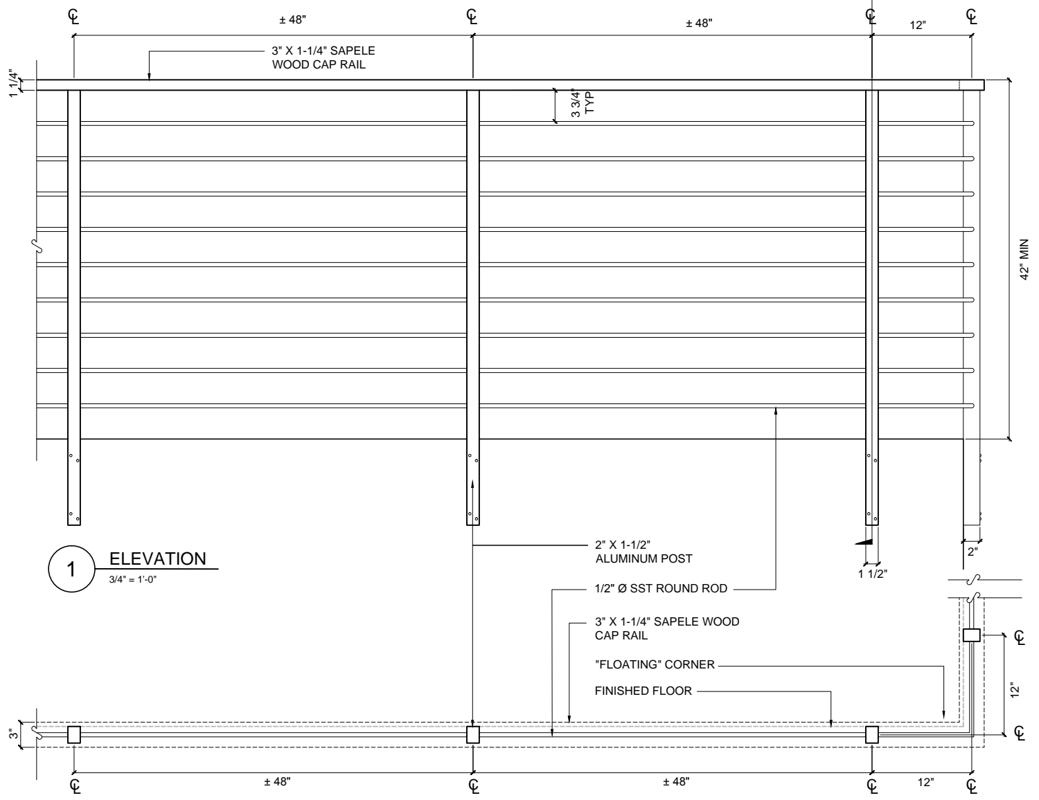
2 PLAN 3/4" = 1'-0"
