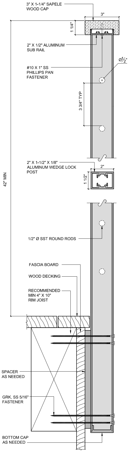
3 SECTION DETAIL - SIDE MOUNT 3" = 1'-0"
