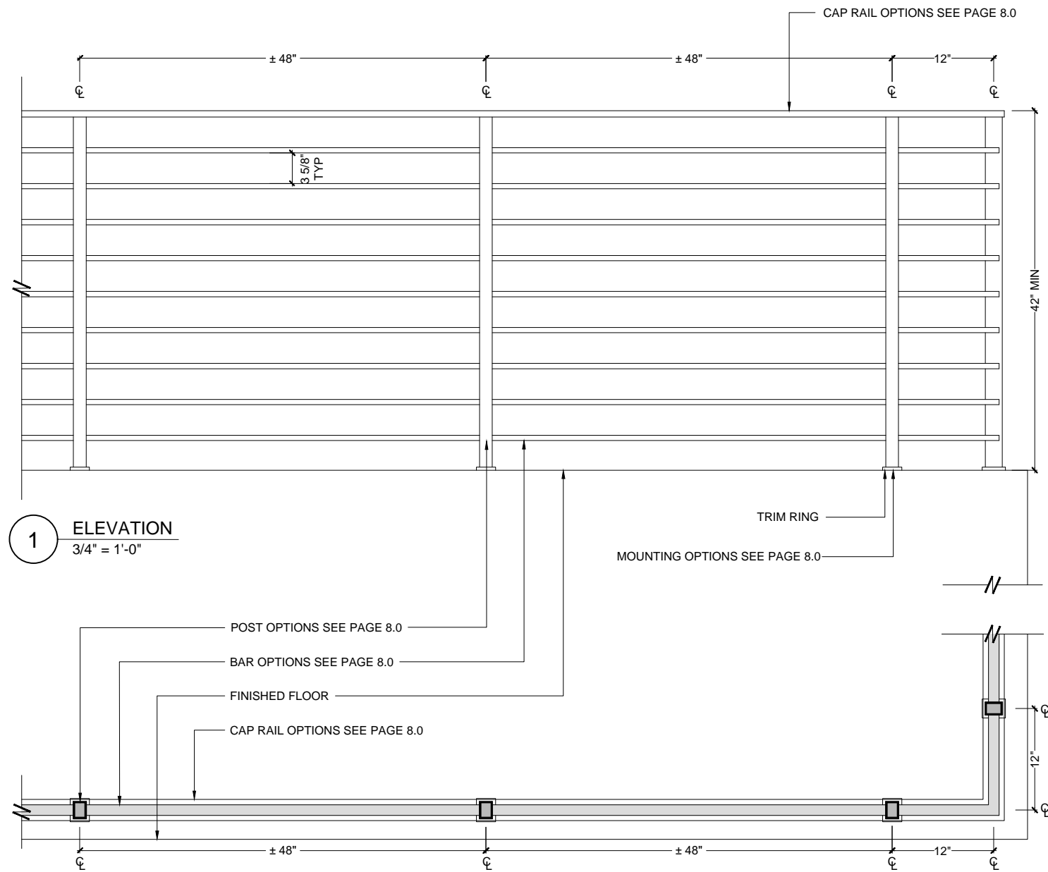
2 PLAN 3/4" = 1'-0"
