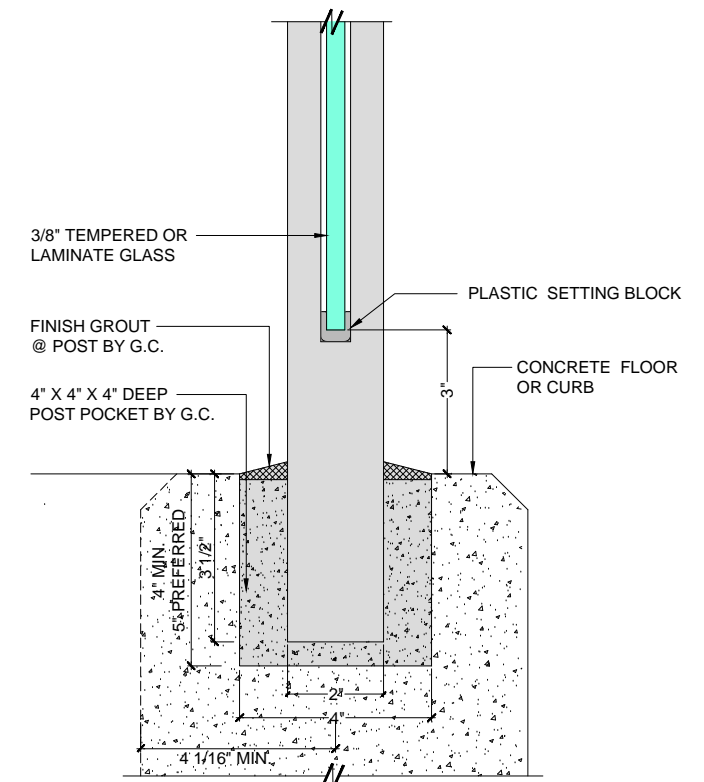
POURED MOUNTING
