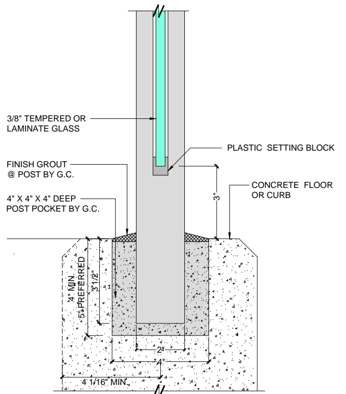
POURED MOUNTING
