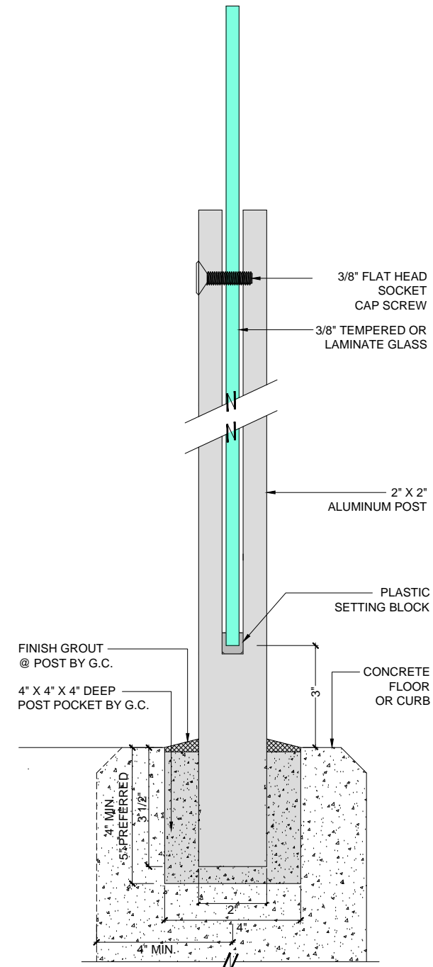
POURED MOUNTING
