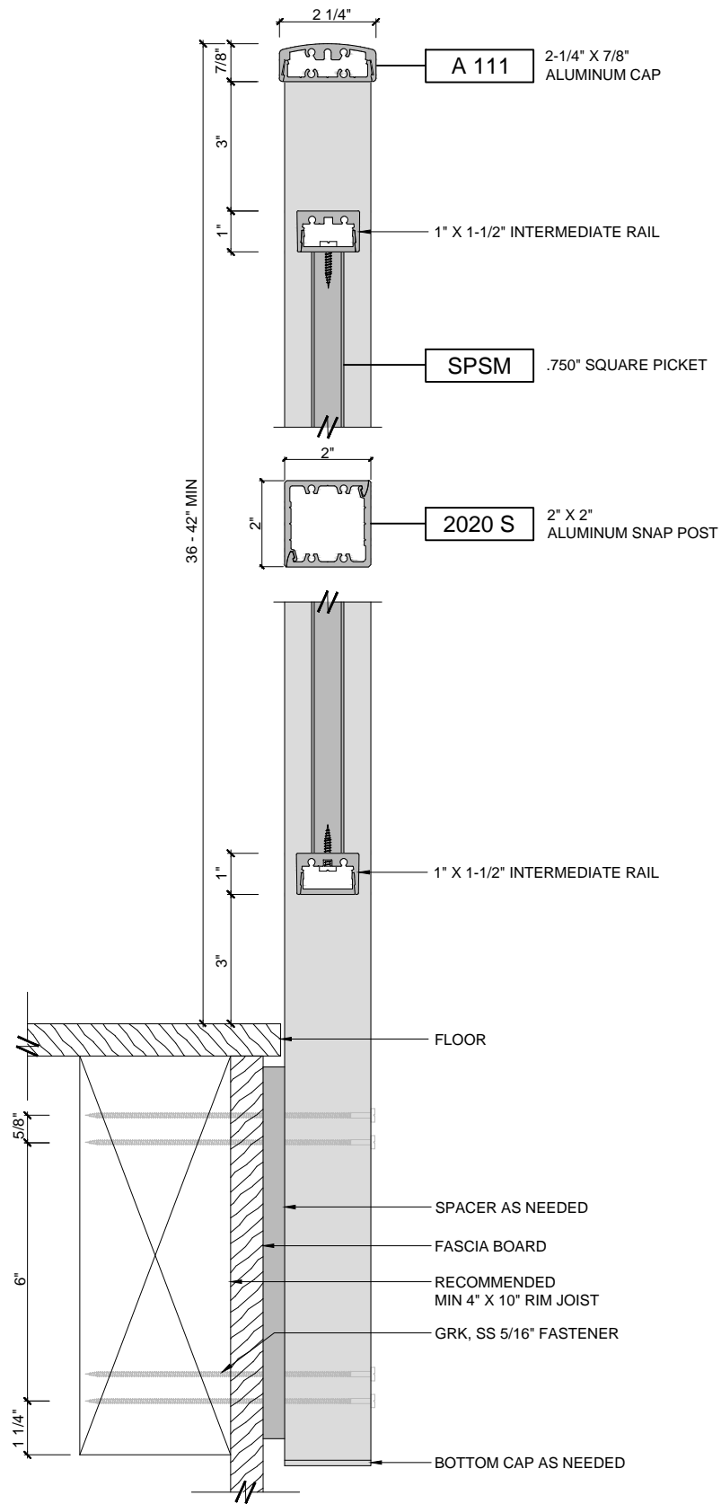
SIDE MOUNTING
