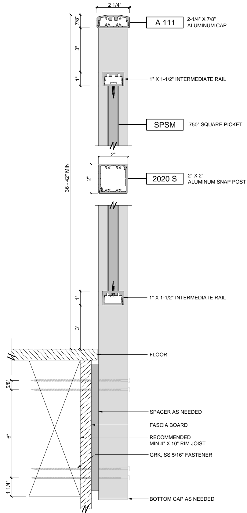
SIDE MOUNTING
