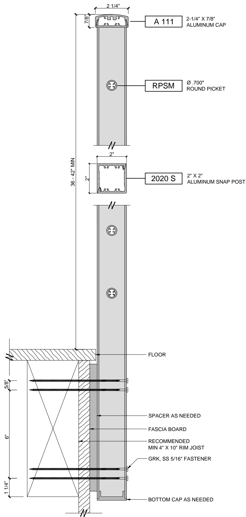
SIDE MOUNTING
