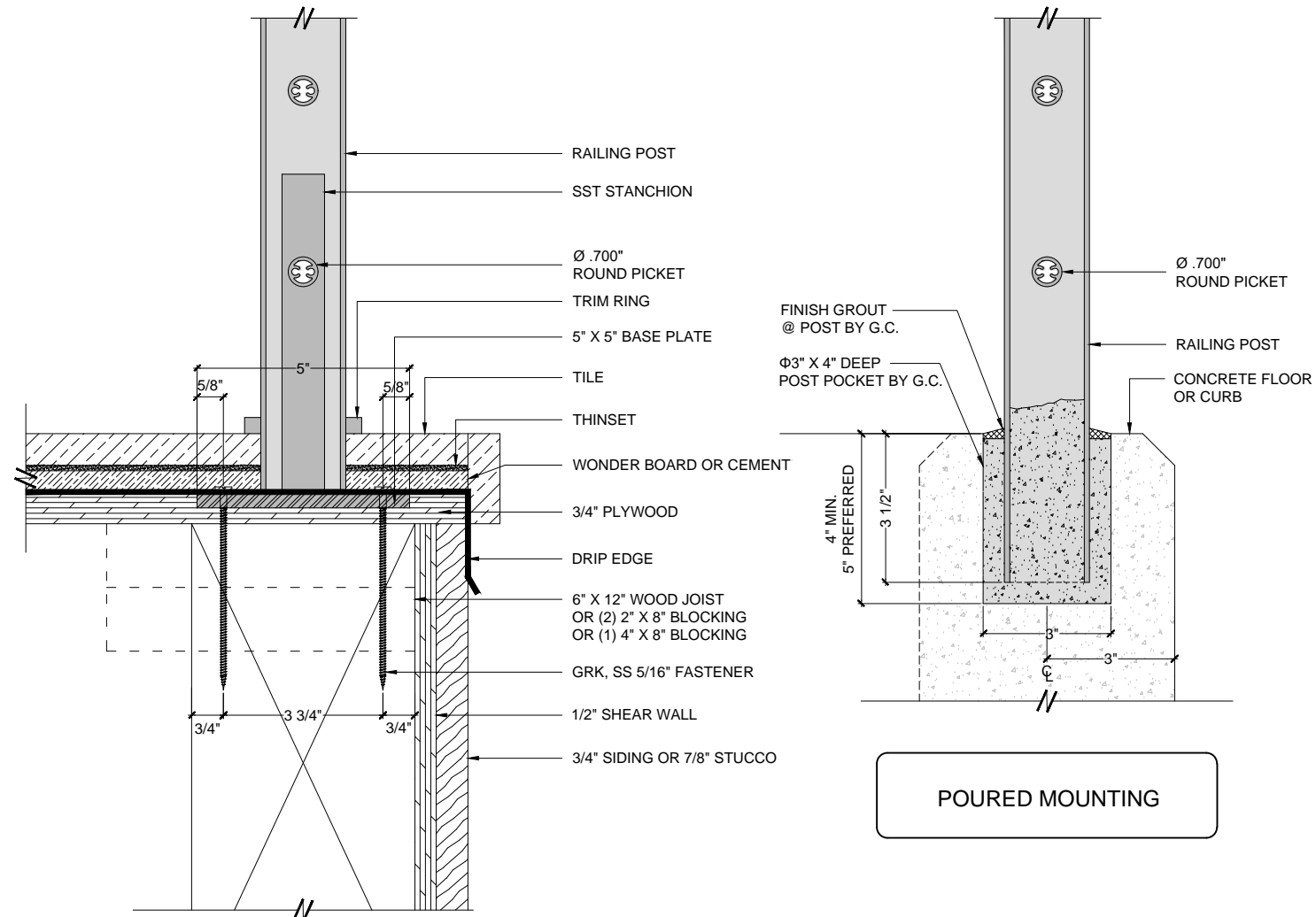
WATERPROOF MOUNTING
