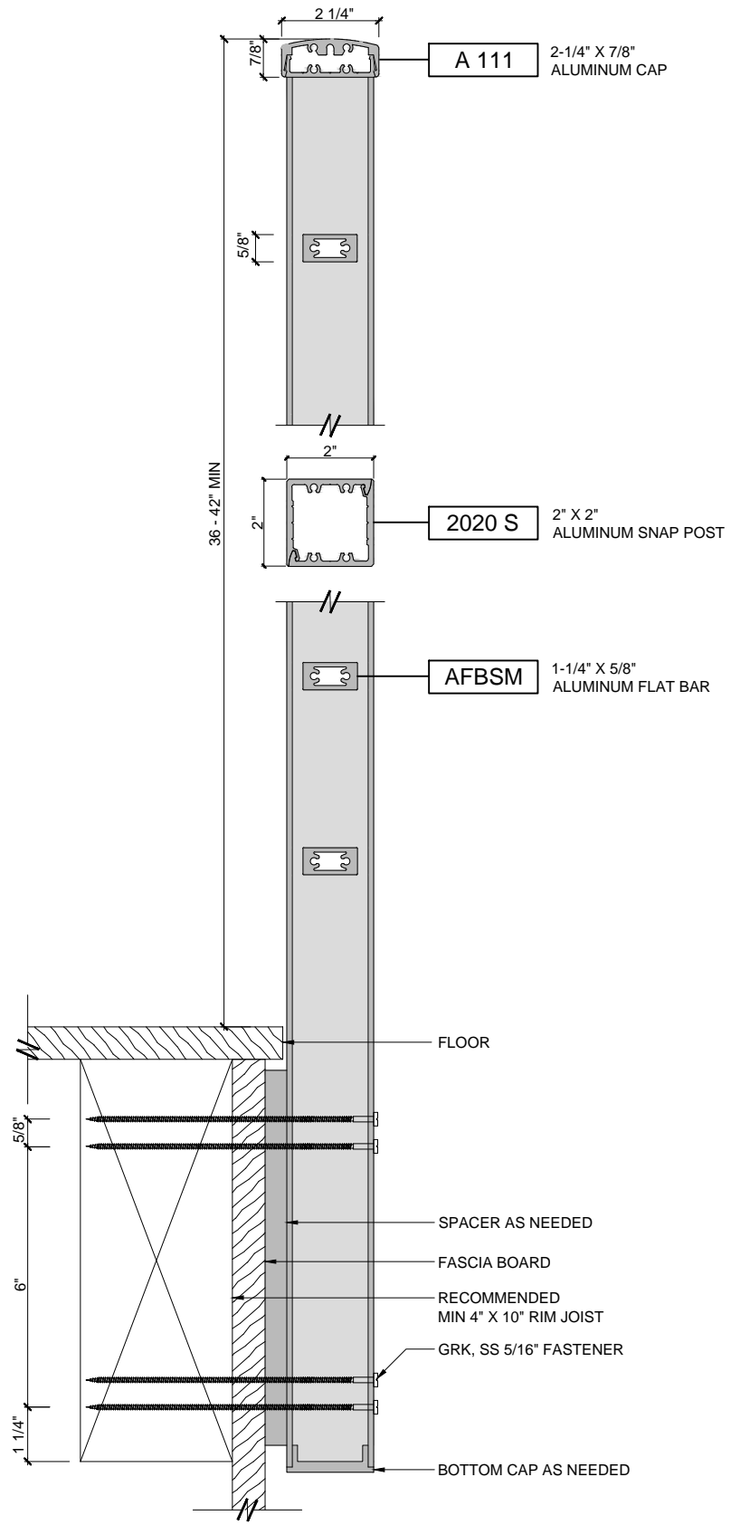
SIDE MOUNTING
