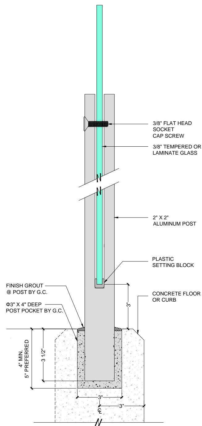
POURED MOUNTING
