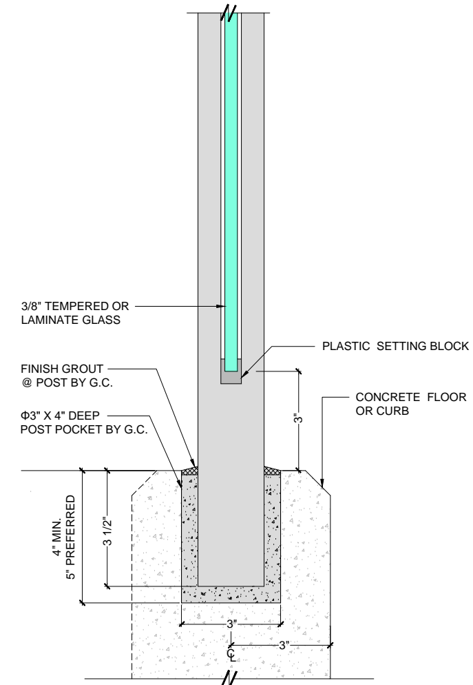
POURED MOUNTING
