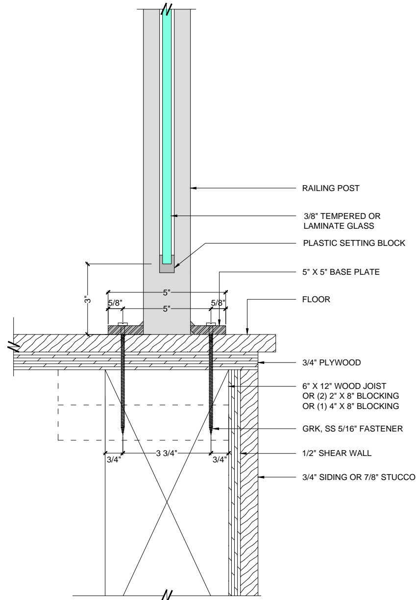
TOP MOUNTING
