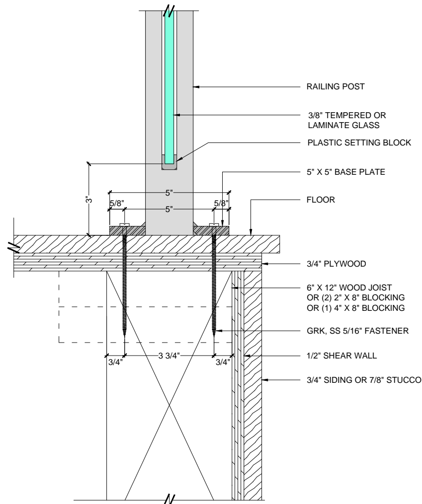
TOP MOUNTING
