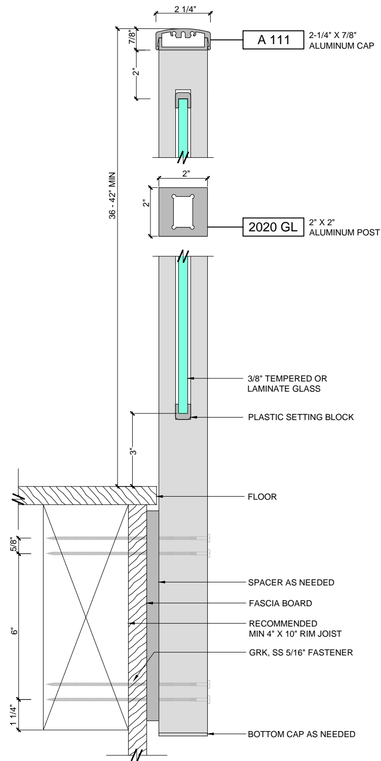
SIDE MOUNTING
