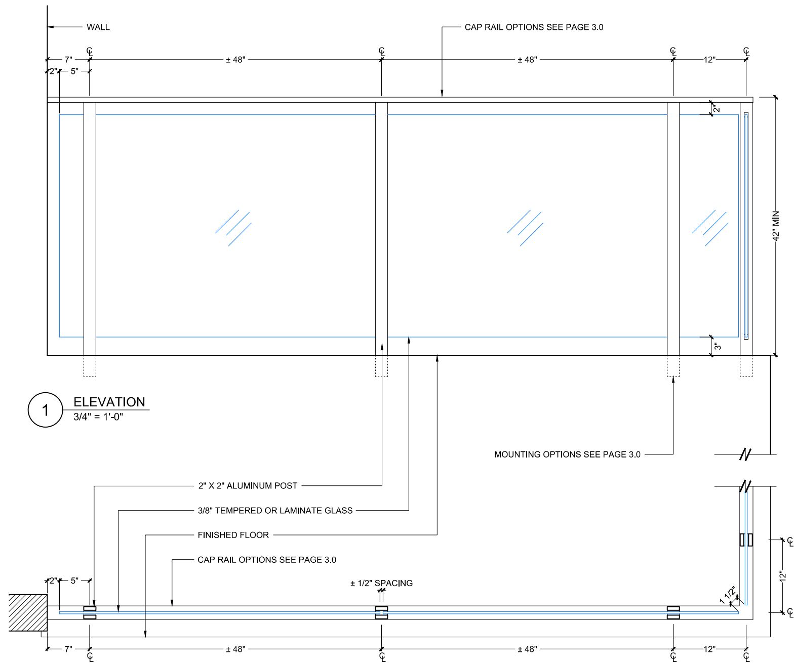
2 PLAN 3/4" = 1'-0"
