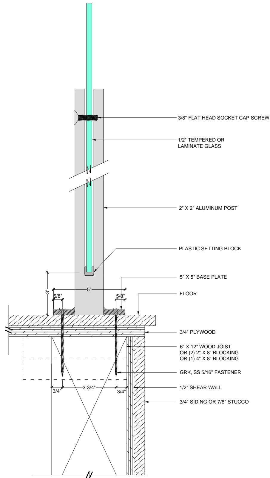
TOP MOUNTING
