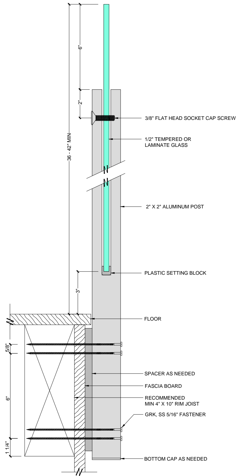
SIDE MOUNTING
