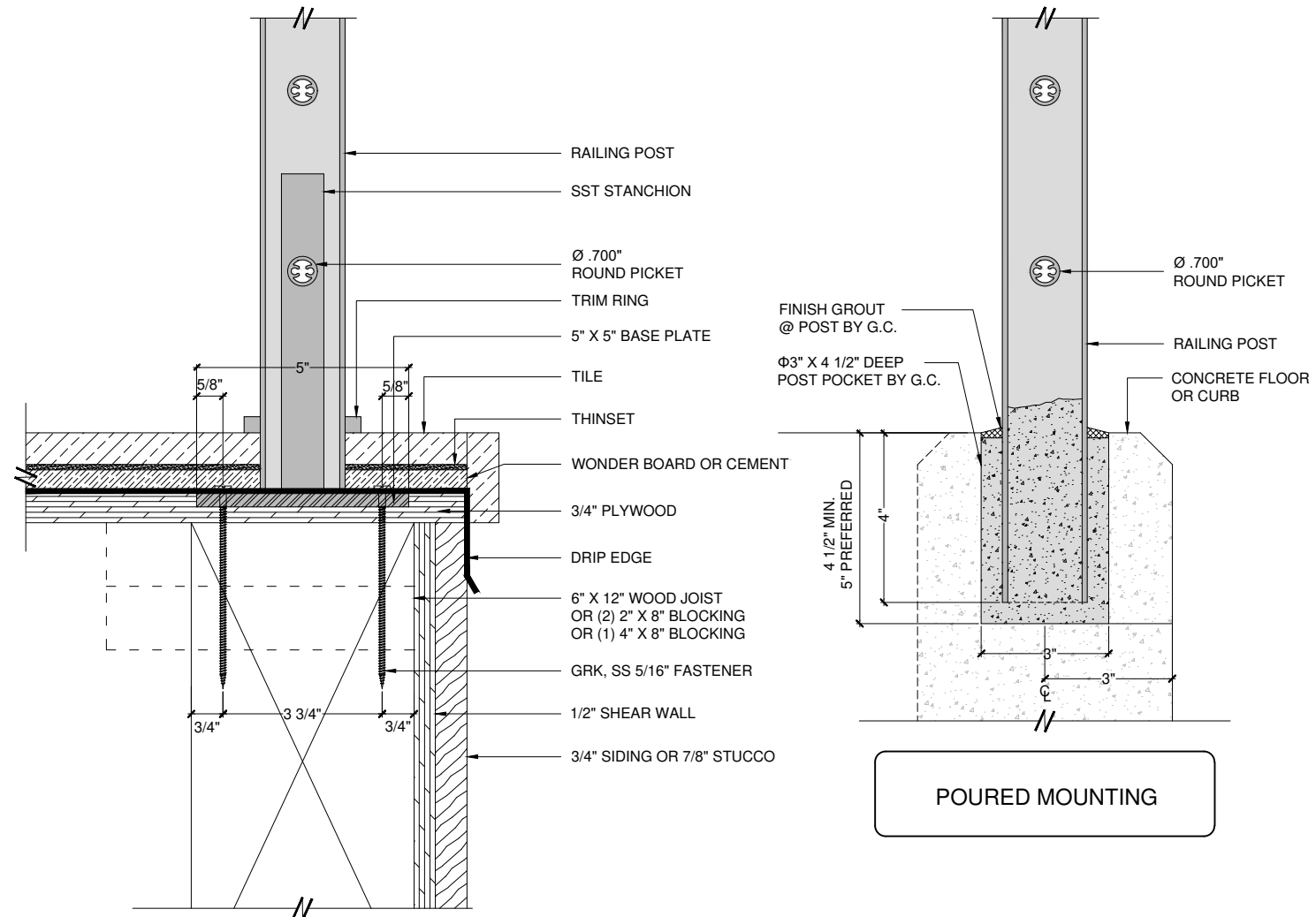
WATERPROOF MOUNTING
