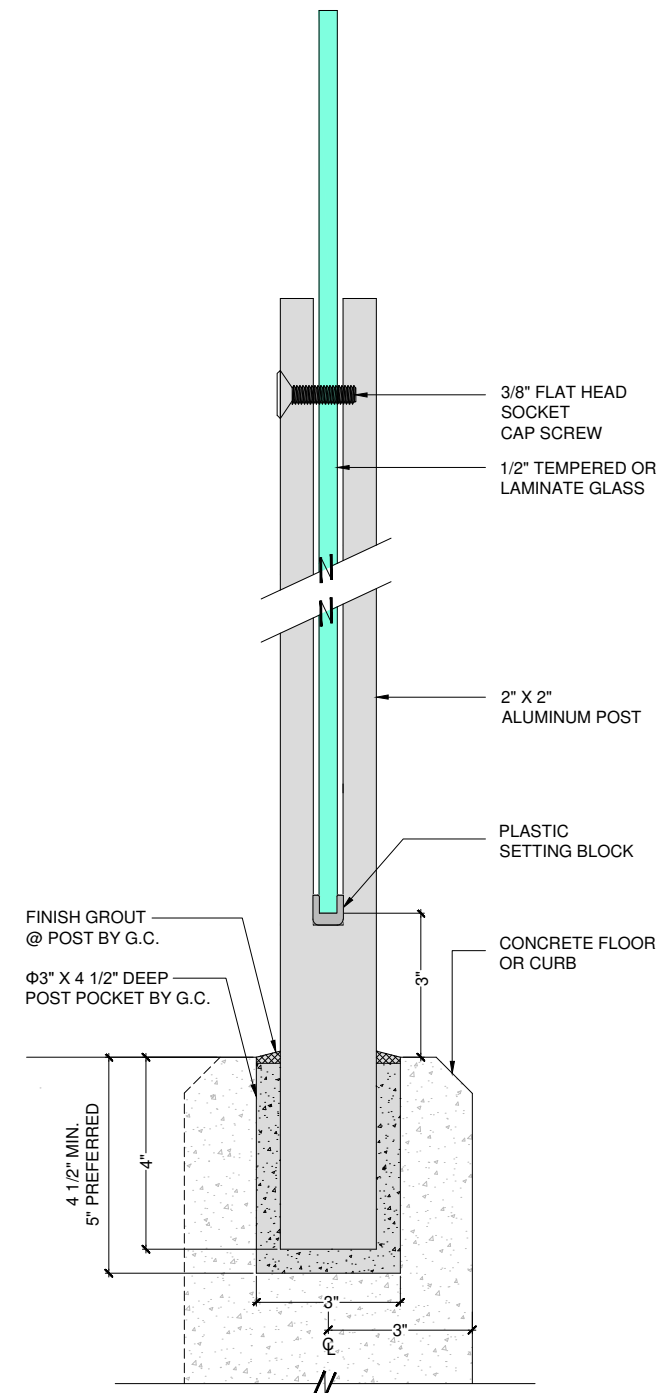
POURED MOUNTING
