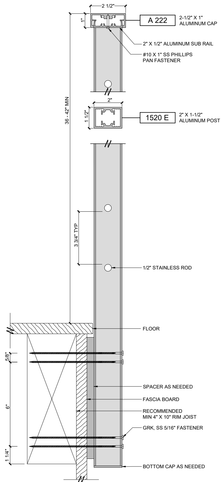
SIDE MOUNTING
