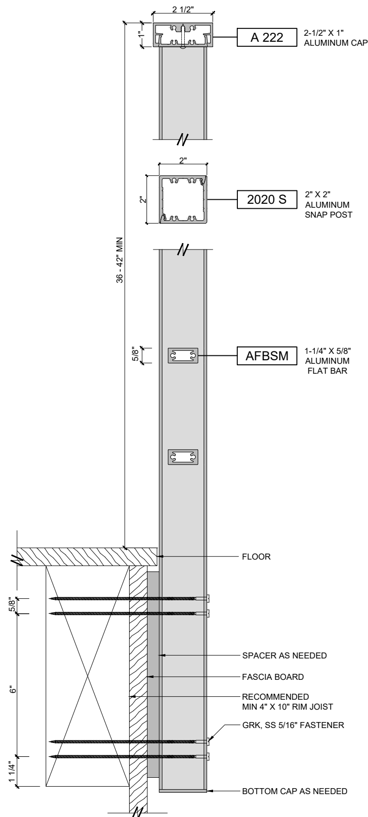
SIDE MOUNTING
