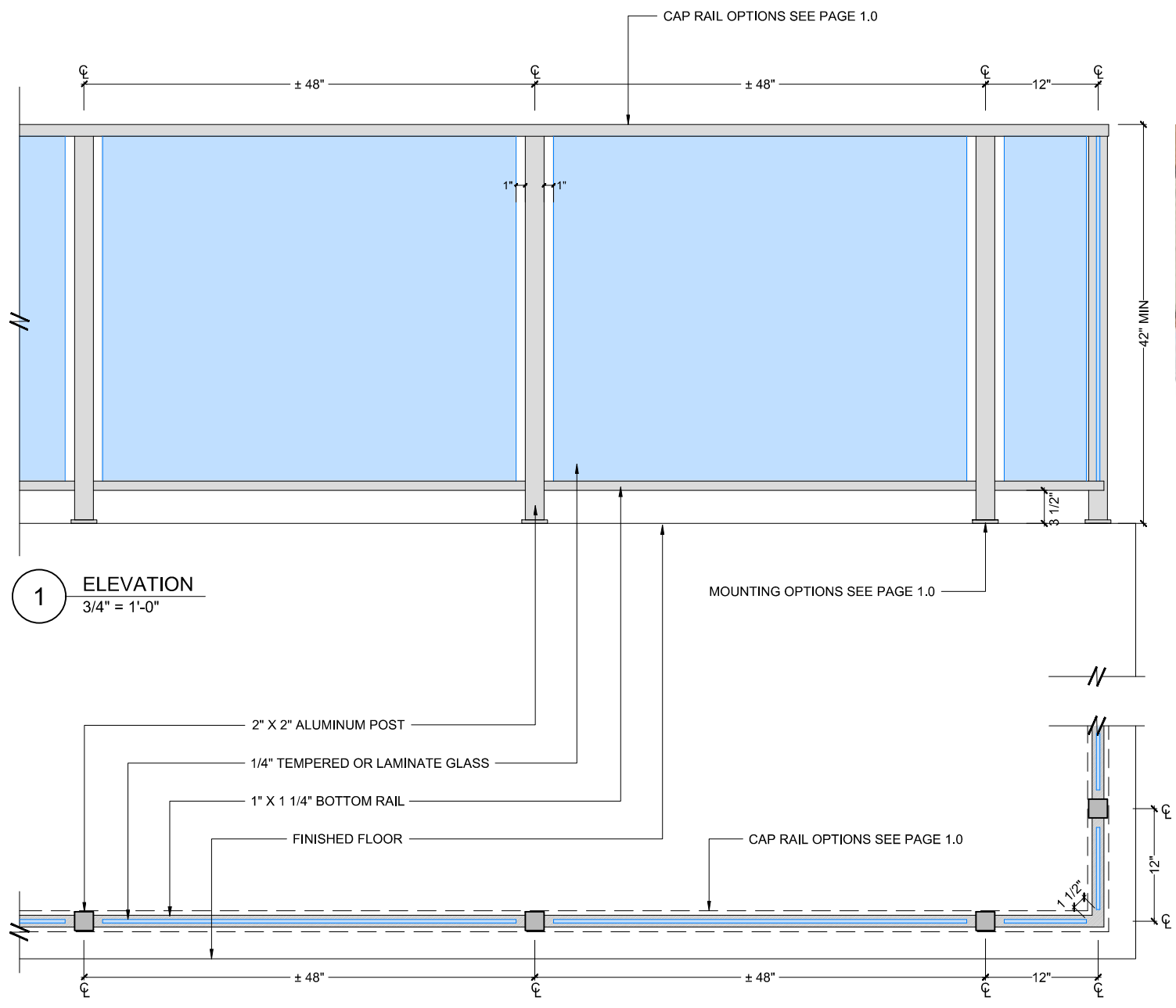
2 PLAN 3/4" = 1'-0"
